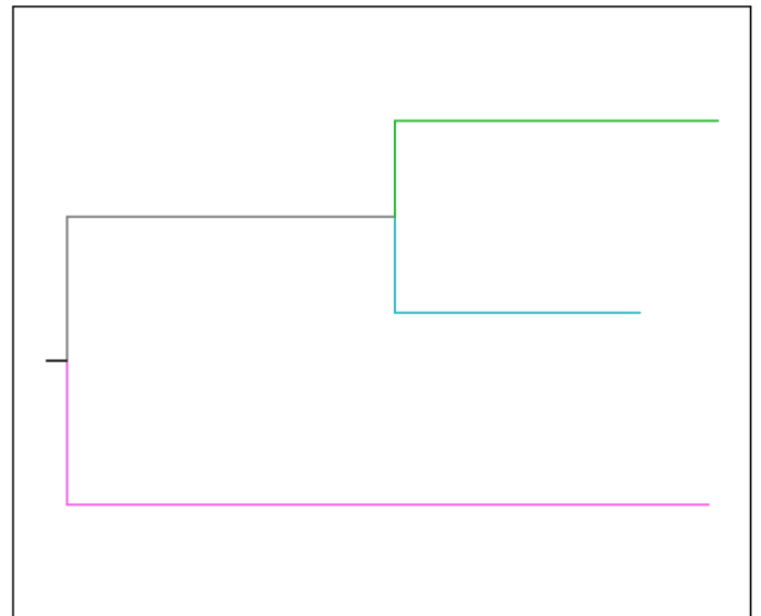
PB2 Subtree 2
